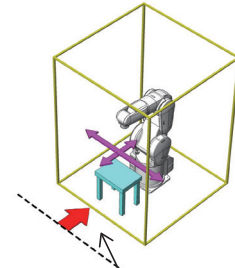
Low monitoring speed set for forward-backward robot movement → Small safe distance (more compact)
