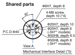
Mechanical Interface Detail (*5)
